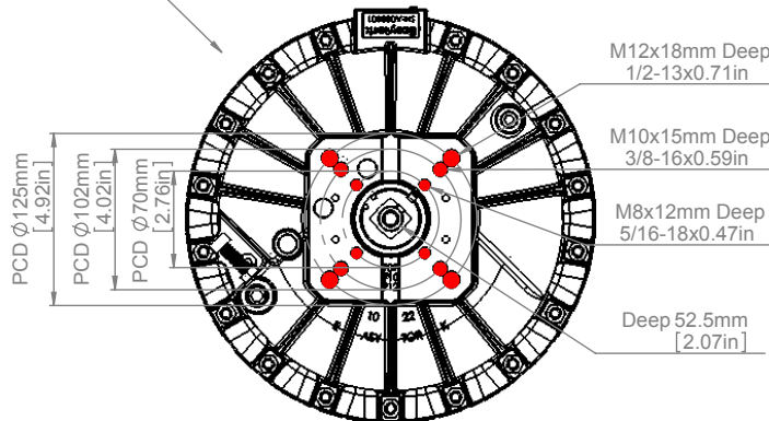
Model 1022 ISO F07/F10/F12 Pattern 0° Shift
