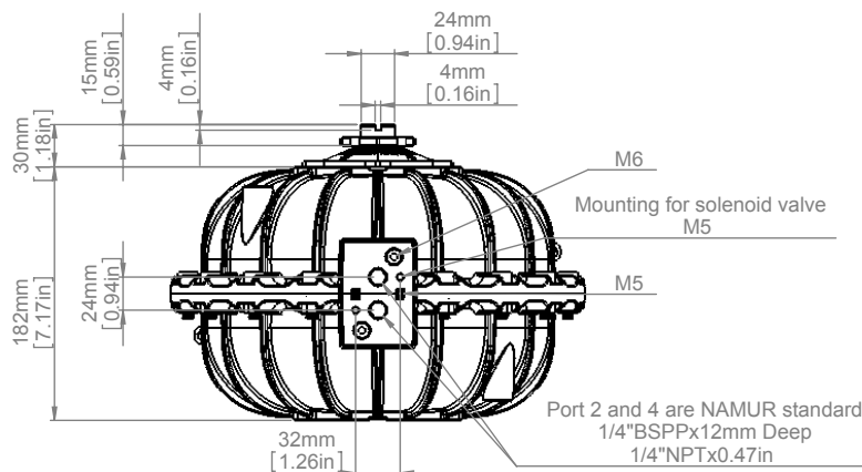
Model 1022 ISO F07/F10/F12 Pattern 0° Shift
