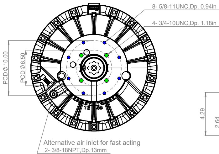
Actuator shown in full CW position Ancillaries attachment size AA3
