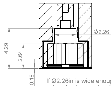
Direct Mount Shaft in EVA (Available Space For Valve Stem)
